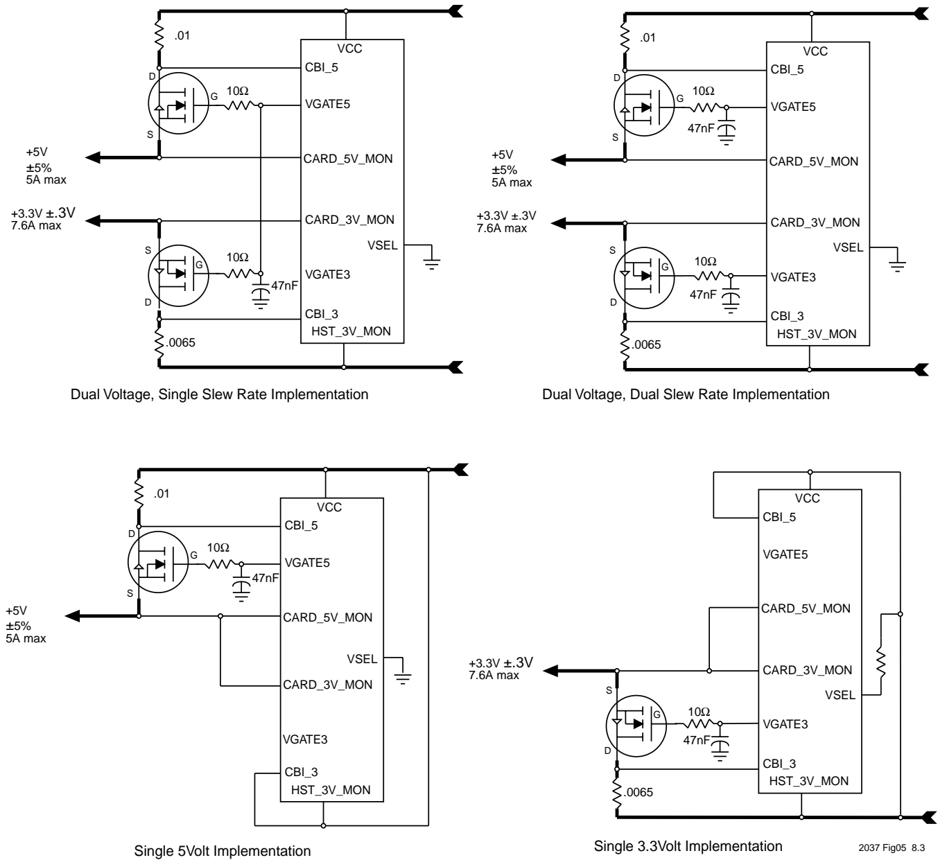
Figure 5. Four power switching implementations
