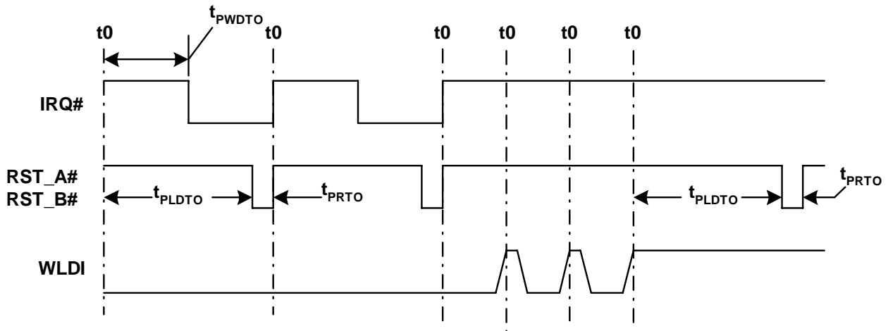
Figure 6. Watchdog, Longdog and WLDI Timing Diagram
