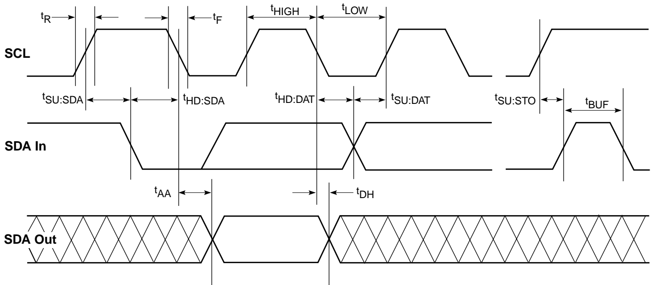
FIGURE 1. BUS TIMING
