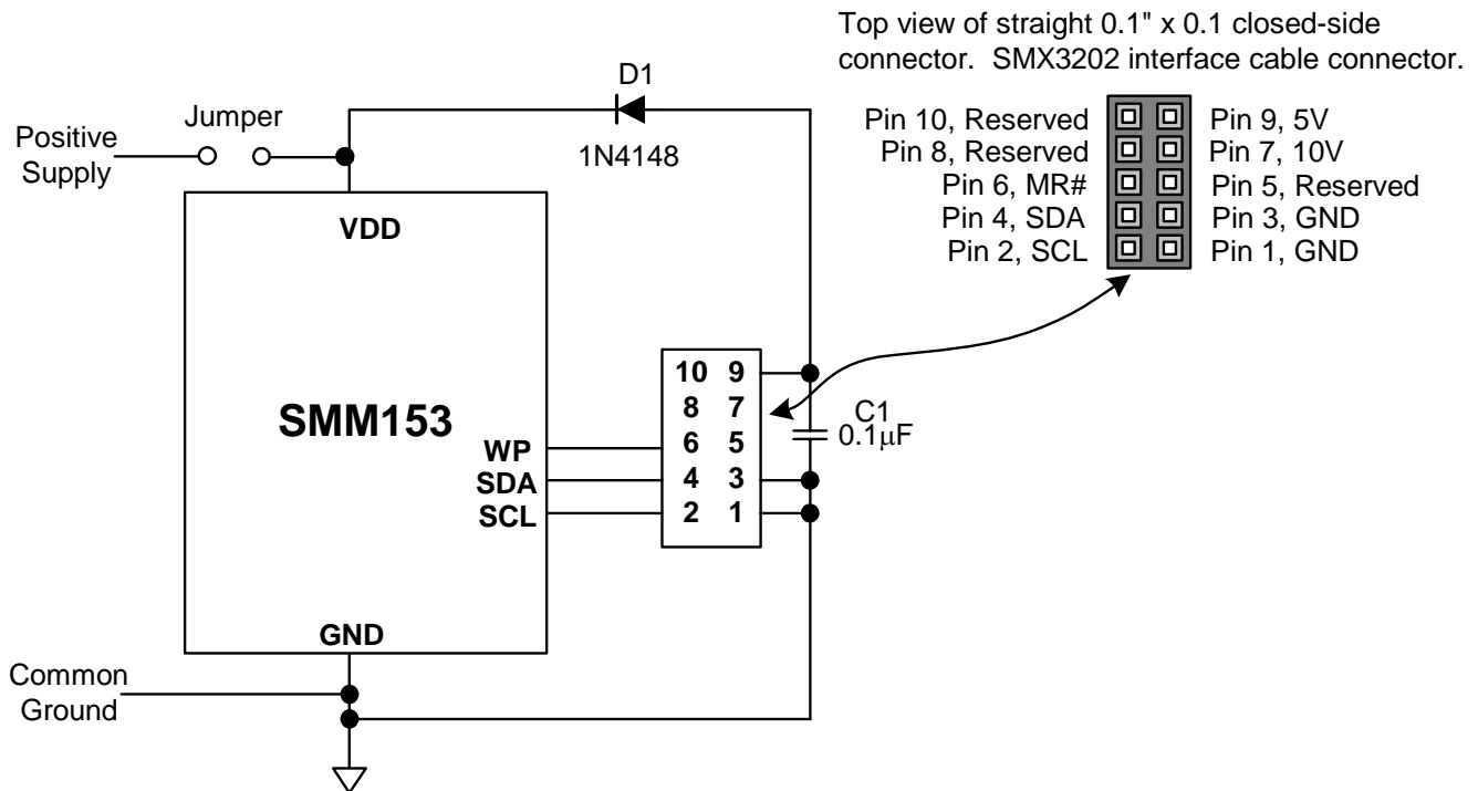
Figure 5 – SMX3202 Programmer I 2 C serial bus connections to program the SMM153. The SMM153 has a Write Protect pin (WP input) which when, asserted, prevents writing to the configuration registers and EE memory. In addition, there is a configuration register lock bit, which, once programmed, does not allow the configuration registers to be changed.
