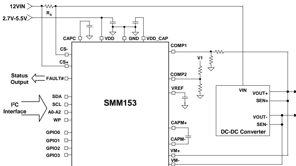
Figure 1 – Application with the SMM153 used to Monitor a DC/DC Converter.
