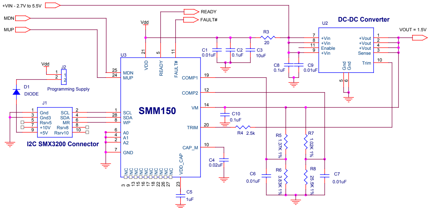
Figure 6 – Typical applications schematic which shows the SMM150 controlling a 3.3V in/1.5V out DC/DC converter. Care should be taken to filter DC/DC converter noise from the SMM150 VDD supply pin. This is accomplished with optional components R3, C1, C2, C3 and C10. This example, using a 1.25V VREF, also shows the COMP1/2 pins monitoring the DC/DC converter VOUT set to an OV of 1.7V on COMP1 and a UV of 1.3V on COMP2, the voltage divider resistors are:
