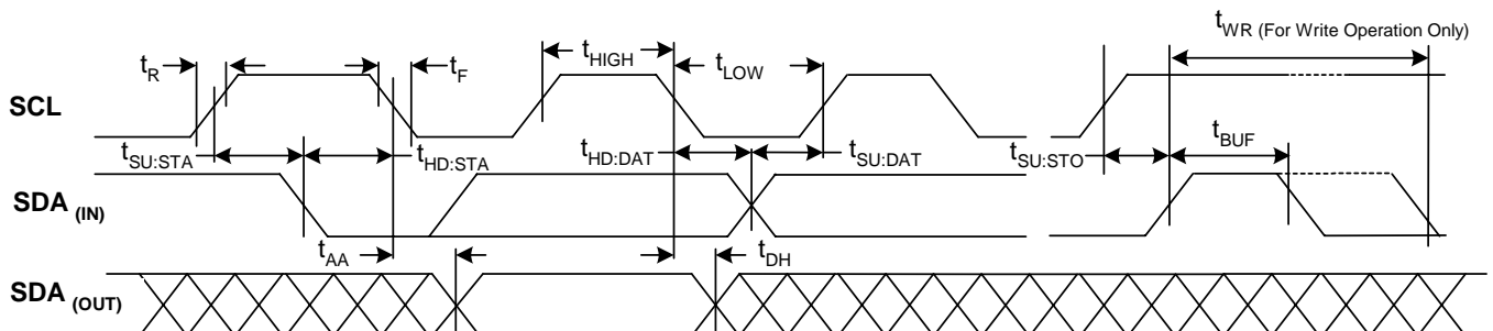
Figure 4 – I 2 C Timing Diagrams
