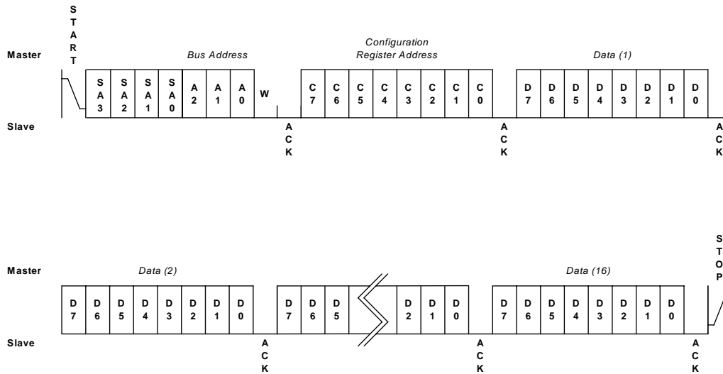
Figure 10 – Configuration Register Byte Write
